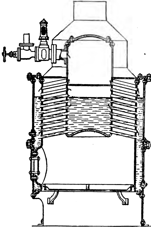
FIG. 156.—One form of the De Dion Tubular Boiler. It consists of an outside annular chamber, forming a waterleg and connected by numerous inclined tubes to the inner steam and water chamber. A partition across this inner chamber secures dry steam for the engine. Steam connections at the top.
